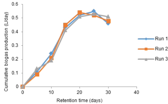
Figure 3. Biogas generation from tea waste
