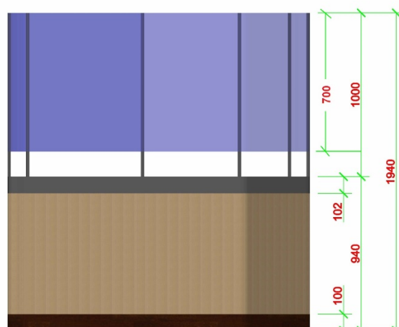
Figure 6. Right View of Proposed Design
