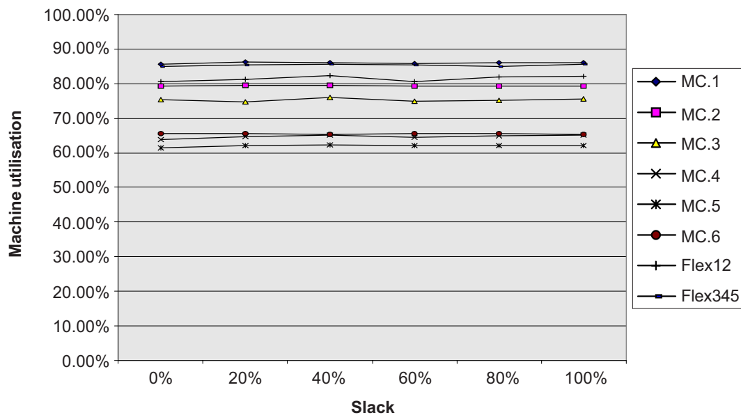
Figure 3 Machine utilisation versus slack (duplication strategy)
